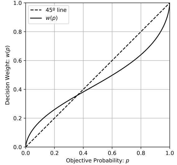
(b) Probability weighting function using the functional form of Equation (8) with \delta = 0.65 .
