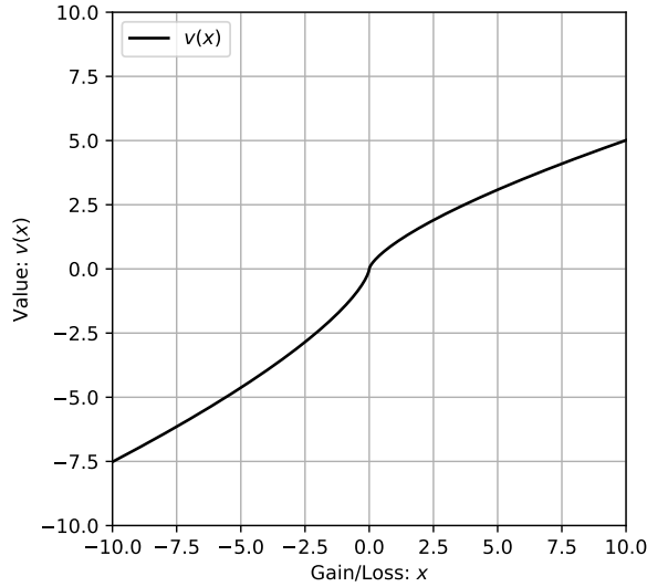
(a) Value function using the functional form of Equation (7) with (\alpha, \lambda) = (0.7, 1.5) .
